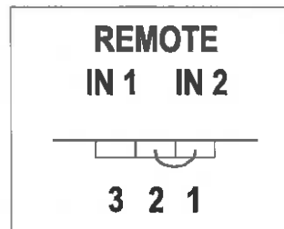
Figure 4: Remote Terminal Block Connector
