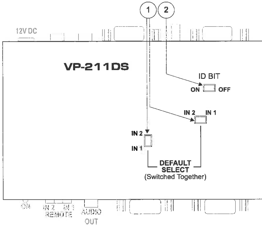
Figure 2: VP-211DS Automatic VGA / Audio Switcher Underside
