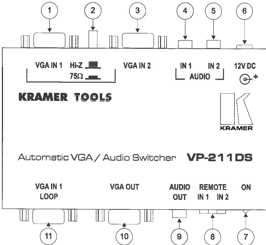
Figure 1: VP-211DS Automatic VGA / Audio Switcher Topside
