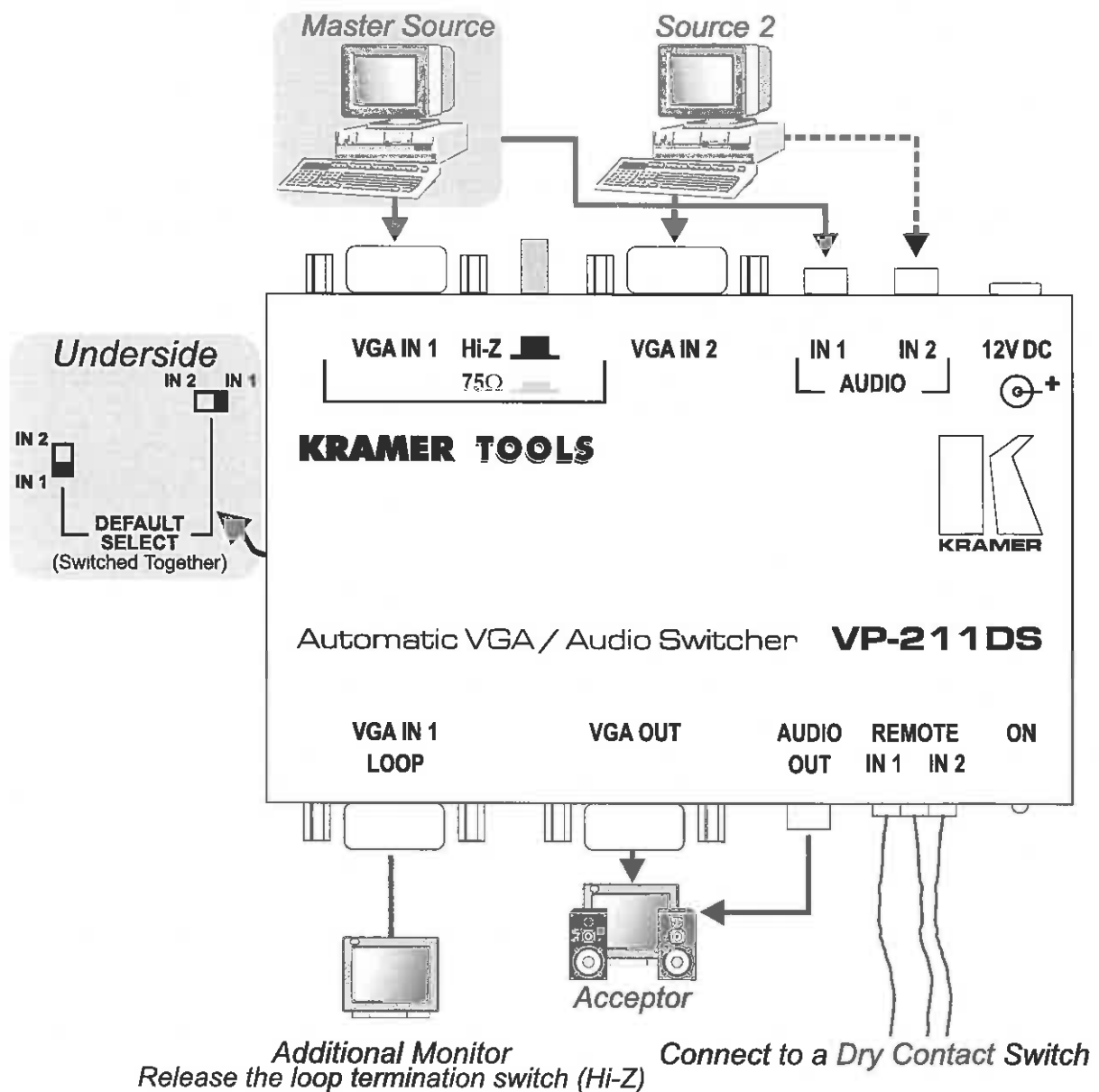
Figure 3: VP-211DS Automatic VGA / Audio Switcher Connections
